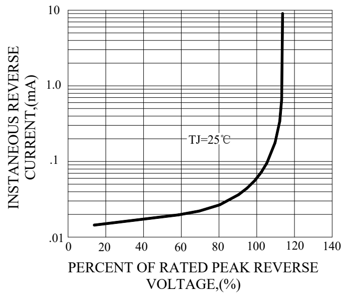
FIG.4-TYPICAL REVERSE CHARACTERISTICS
