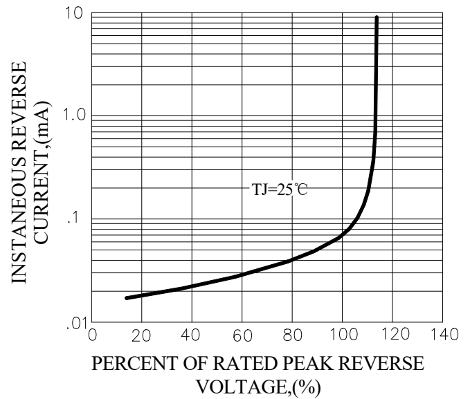
FIG.4-TYPICAL REVERSE CHARACTERISTICS
